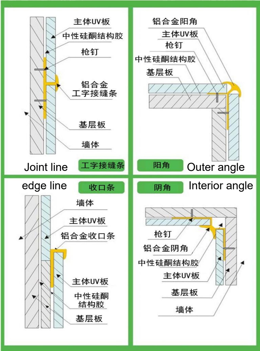
铝合金外角- (阳角) Aluminum alloy line - outer angle
