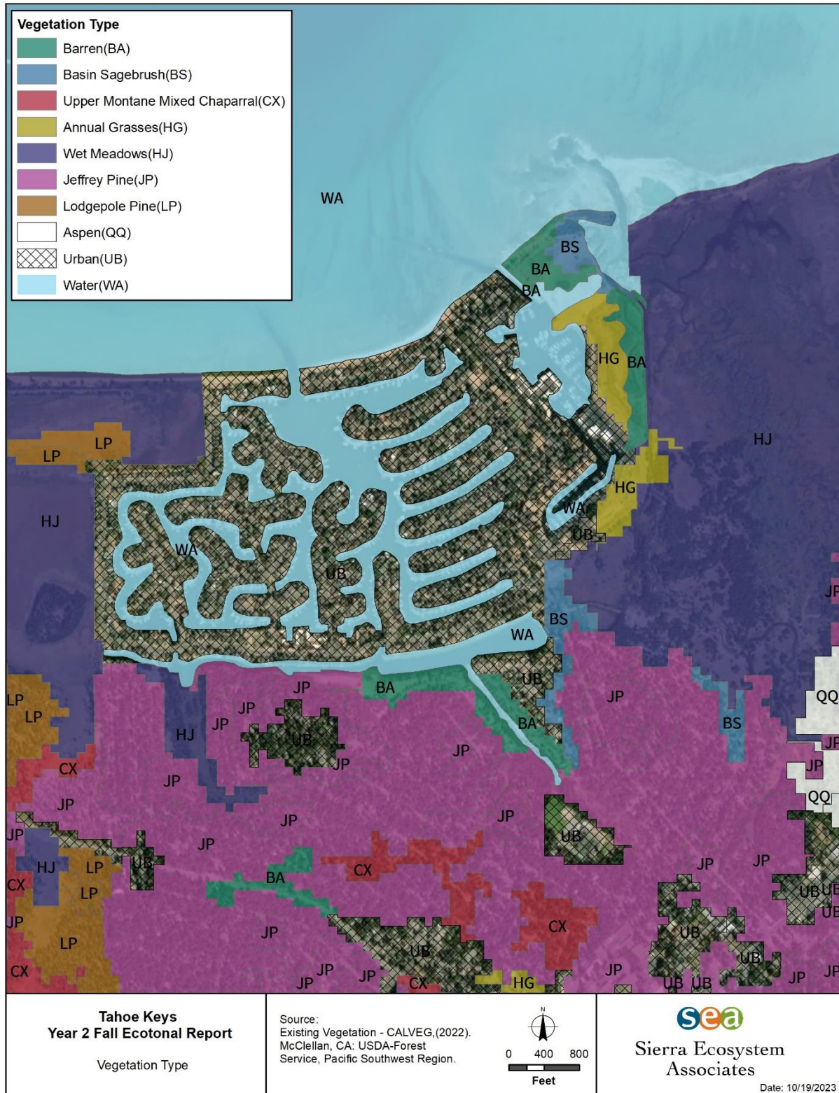
Figure 3. Vegetation Classification
