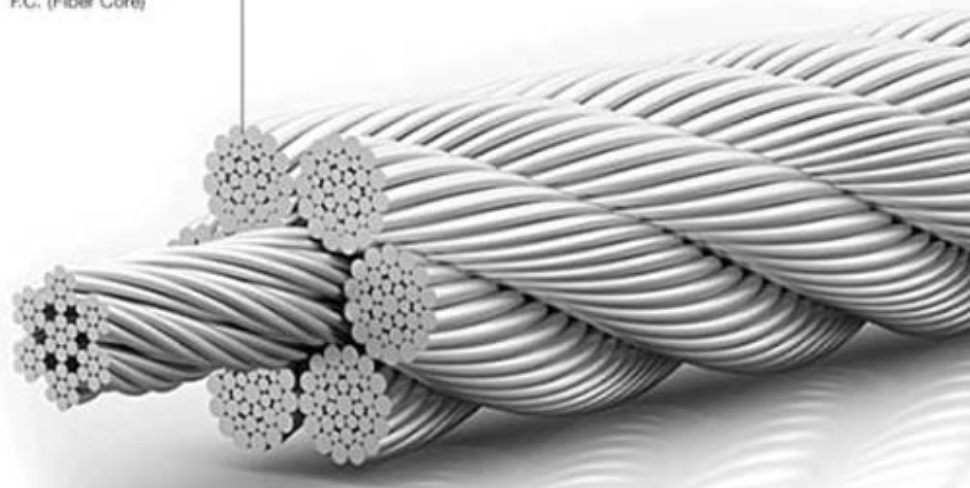
6x36 Warr. Seale F.C. (Fiber Core)
