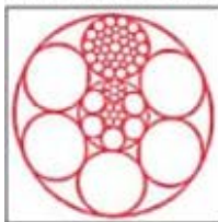
6x36 Warr. Seale IWRC (Steel Core)
