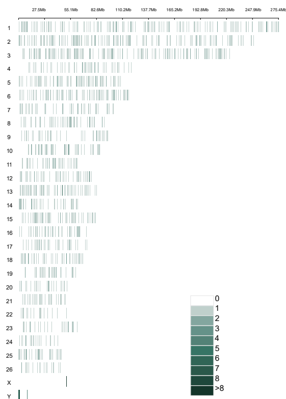
Figure 1 Distribution of target SNP sites on chromosomes
