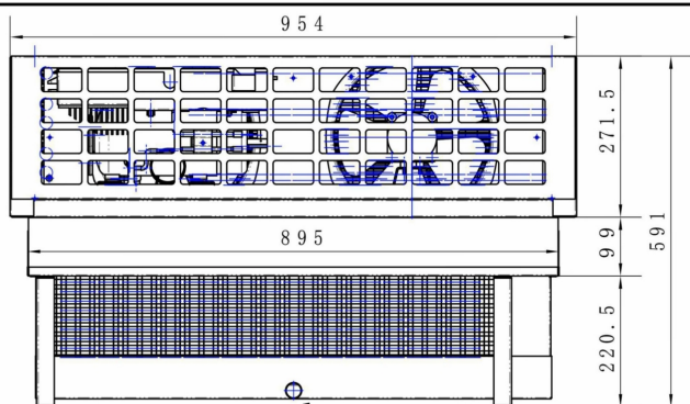
Condensate Drainage
