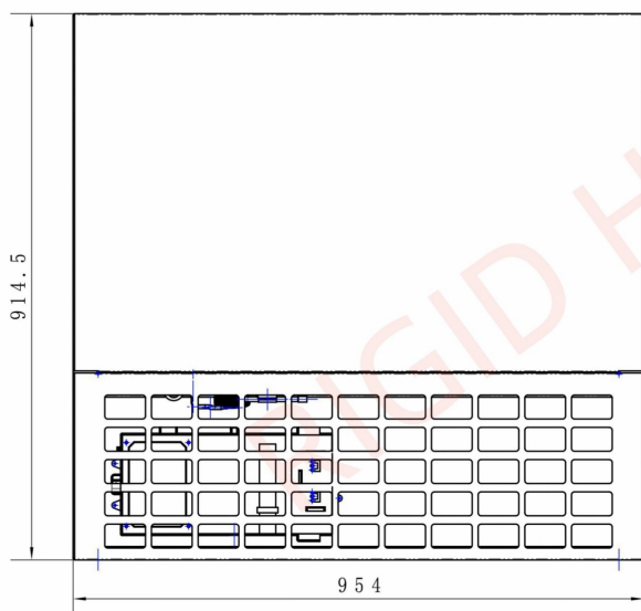
Condensate Drainage
