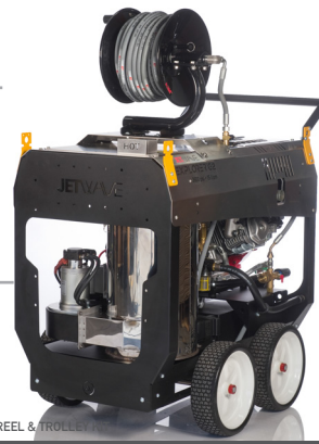
SHOWN WITH OPTIONAL HOSE REEL & TROLLEY KIT
