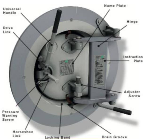
Horizontal Closure Components
