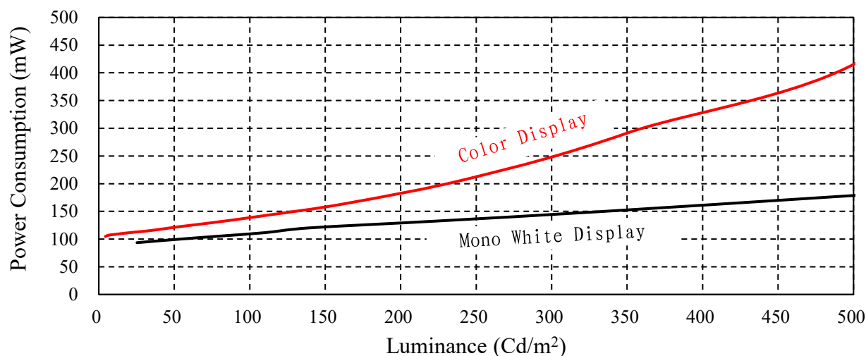
Figure 5-5 SVGA097 Power consumption characteristic with luminance
