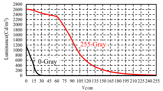
Figure 5-2 Monochrome White Display
