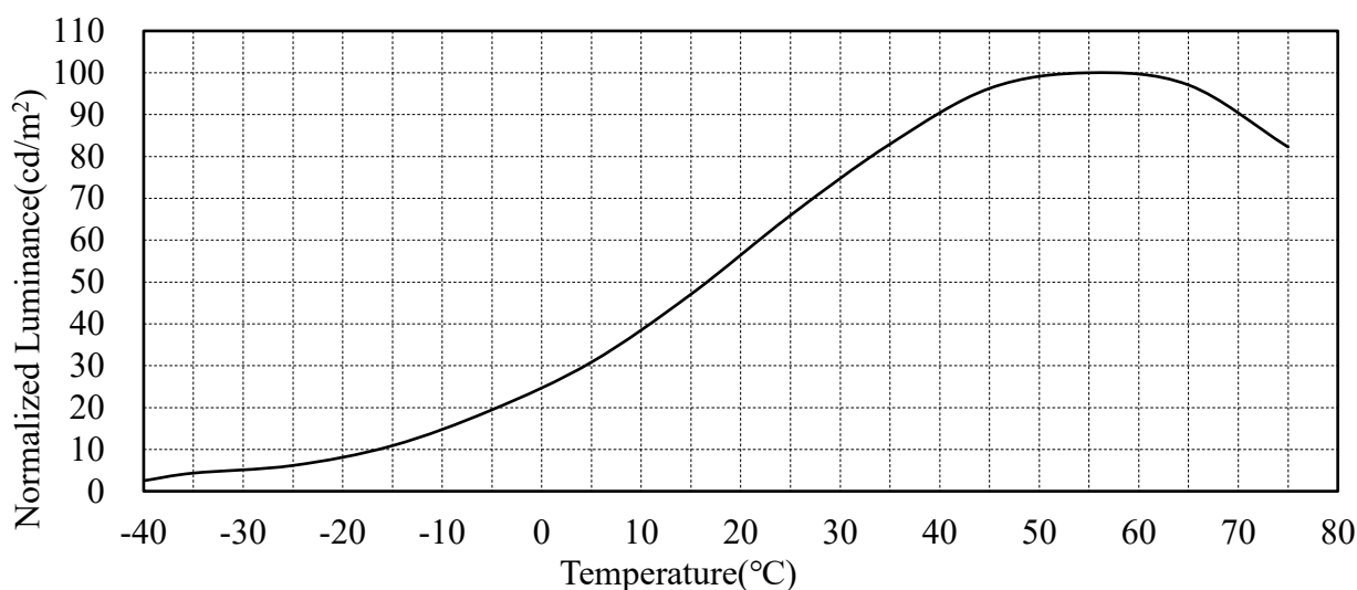
Figure 5-4 SVGA097 Luminance characteristic curve with temperature
