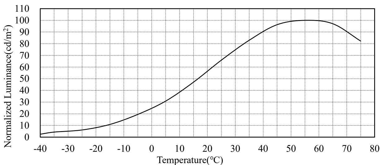
Figure 5-4 SVGA060 Luminance characteristic curve with temperature
