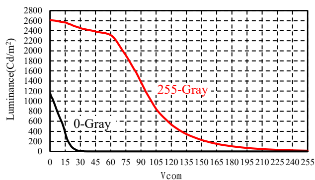
Figure 5-2 Monochrome White Display
