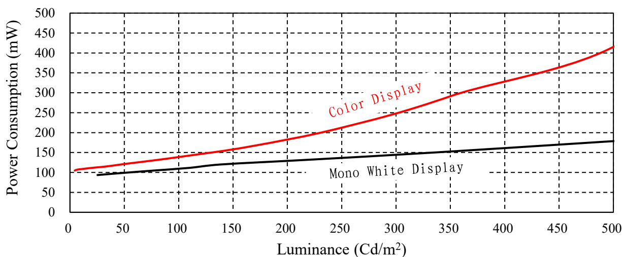
Figure 5-5 SVGA060 Power consumption characteristic with luminance
