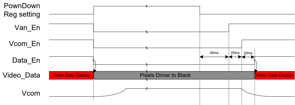
Figure 3-11 Register Control Power Down & Up
