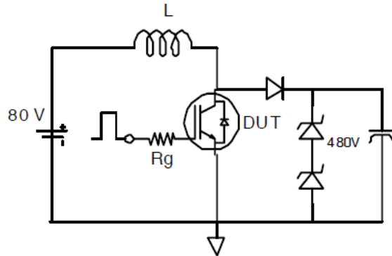
Fig.10 RBSOA Circuit
