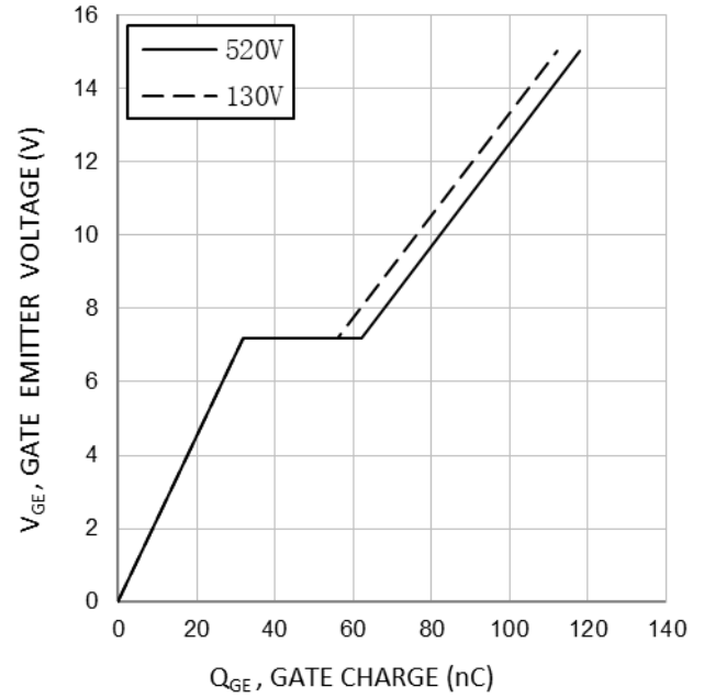
Fig. 14 Typical gate charge ( I_C=75\text{A} )
