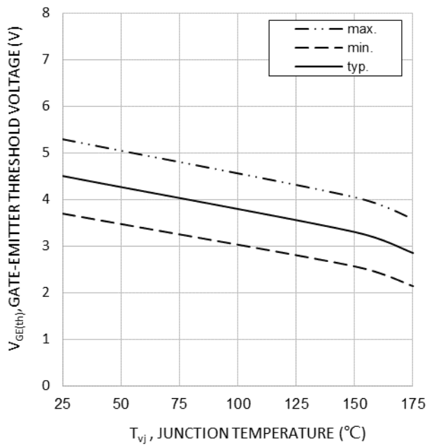
Fig. 5 Gate-emitter threshold voltage as a function of junction temperature ( I_c=0.40mA )
