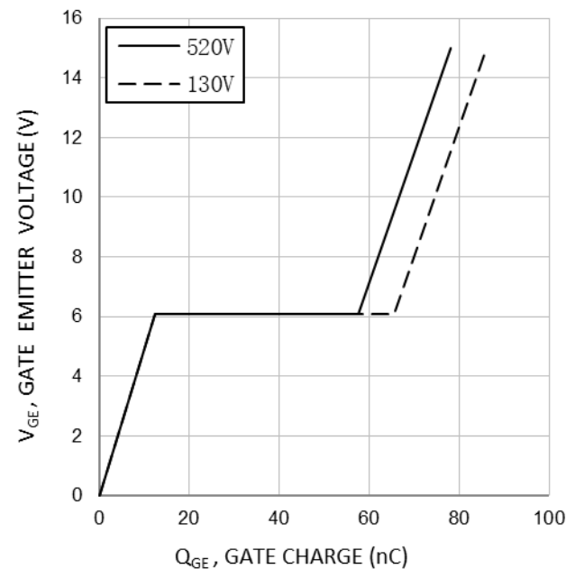
Fig. 8 Typical gate charge ( I_c=50A )
