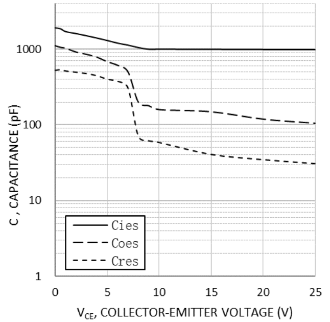
Fig. 6 Typical capacitance as a function of collector-emitter voltage ( V_{GE}=0V , f=1MHz )
