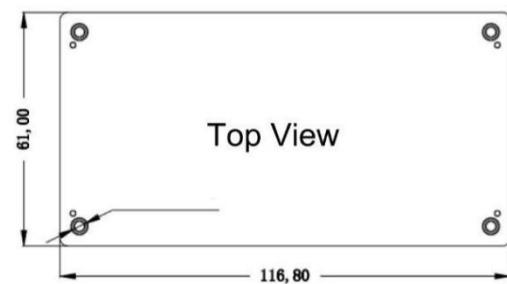
Standard 116.8*61*12.5mm
