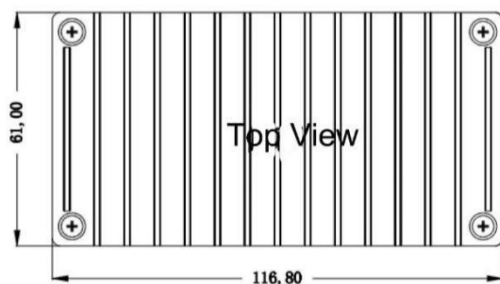
Standard+Heatsink 116.8*61*32.5mm
