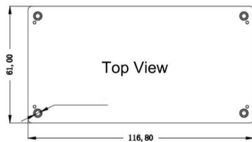
Standard 116.8*61*12.5mm
