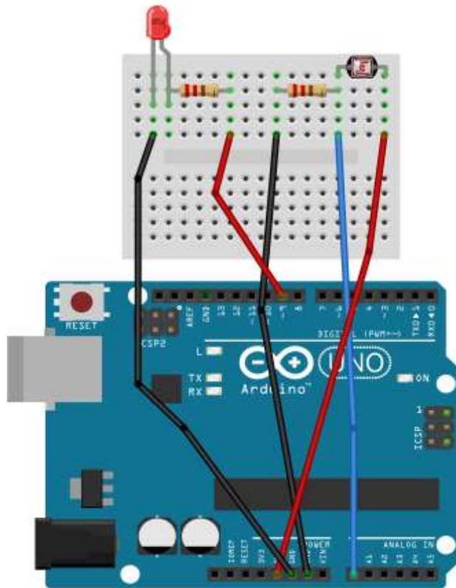
Figure 1: Hardware Set-Up for LDR (Light Dependent Resistor) Exercise
