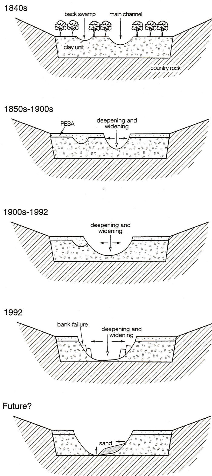
Figure 15. Changes in Channel Morphology since European Settlement
