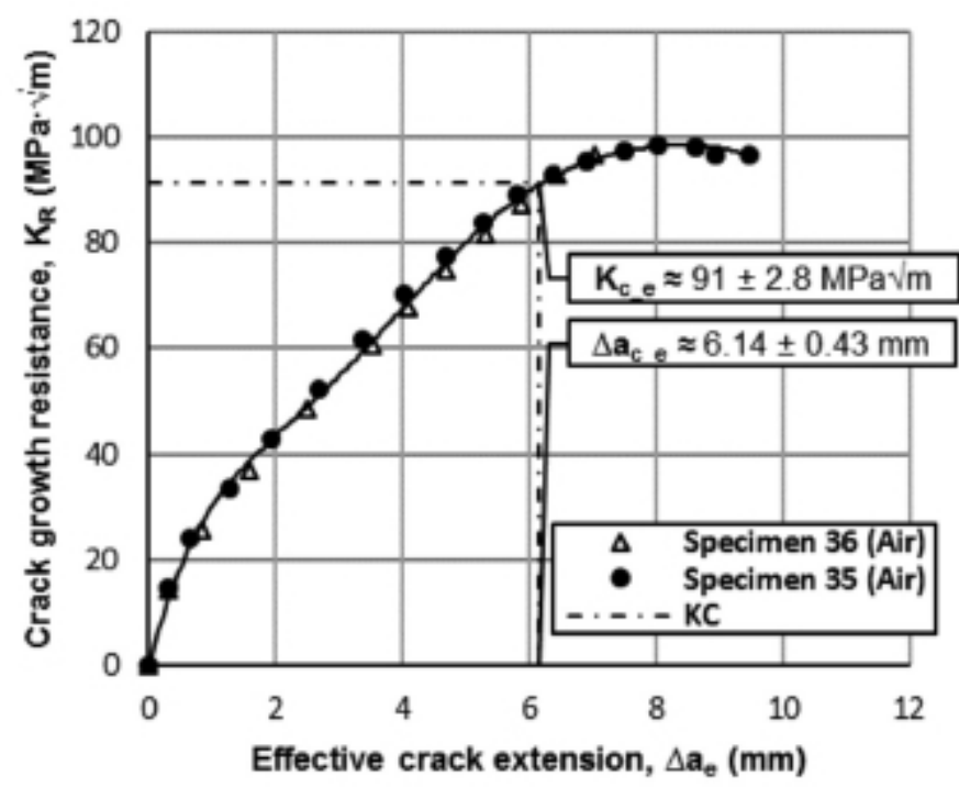
Figure 5—The apparent crack growth resistance behaviour of 3.2 mm thick aluminium alloy 2024-T3 after prior exposure to air (baseline results)
