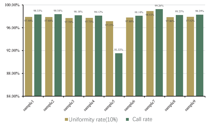
Figure 2 Uniformity(10%) and detection rate of performance in different samples
