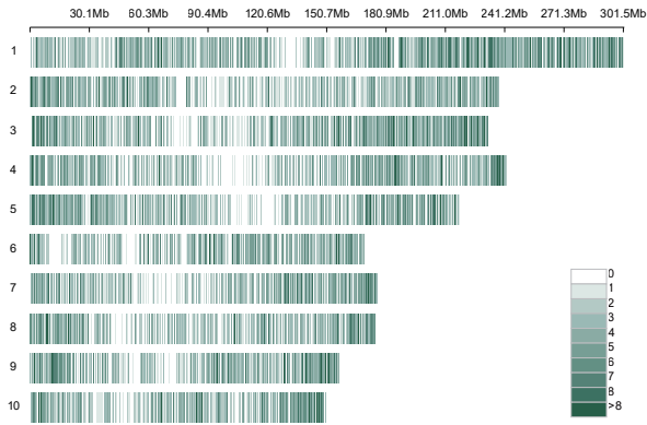
Figure 1 Distribution of SNP numbers on chromosomes
