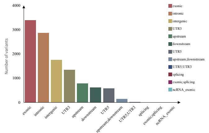
Figure 4 Annotation of SNP
