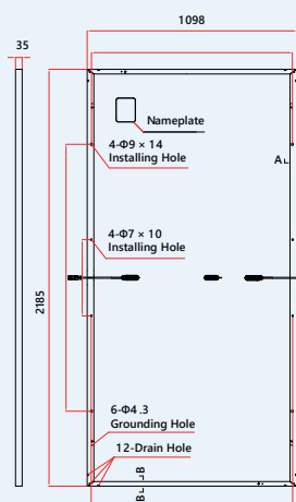
Back View
