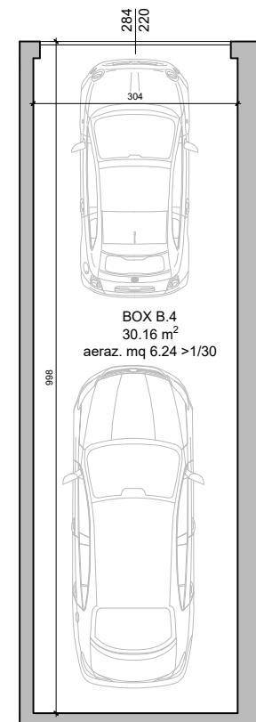
PIANO INTERRATO
