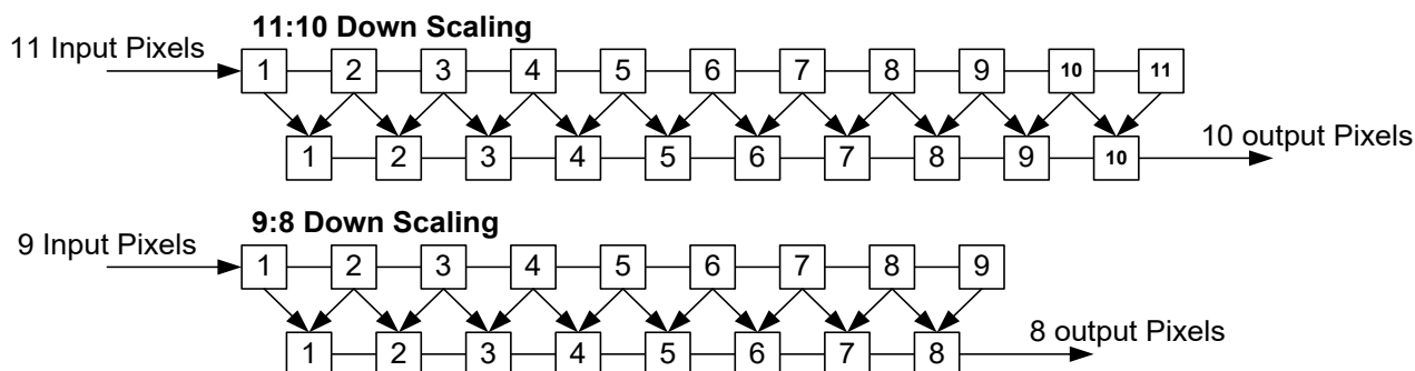
Figure 3-4 Diagram of the Horizontal Scaling Algorithm
