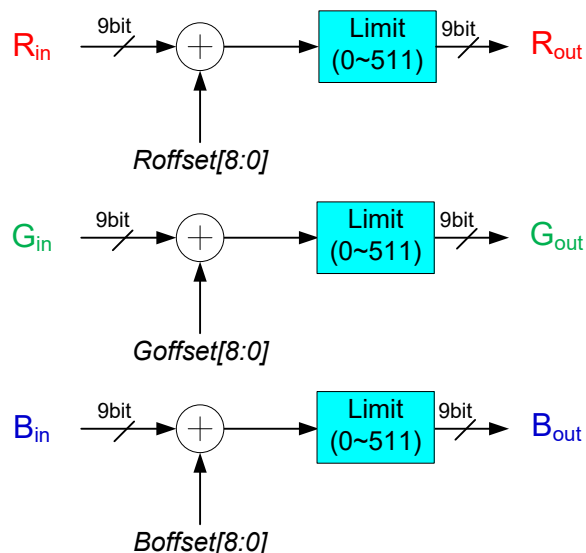
Figure 3-7 Color Offset Control
