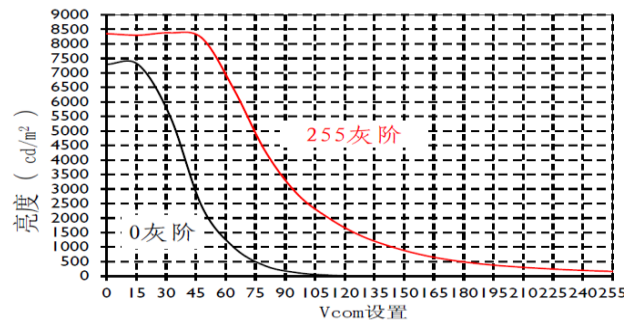
Figure 5-3 Monochrome Green Display
