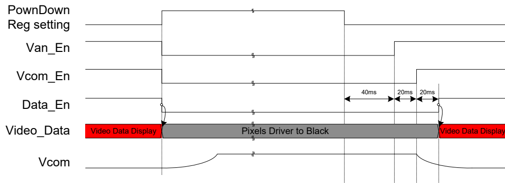
Figure 3-11 Register Control Power Down &amp; Up
