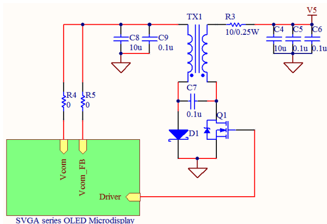
Figure 3-16 DC/DC Principal Diagram
