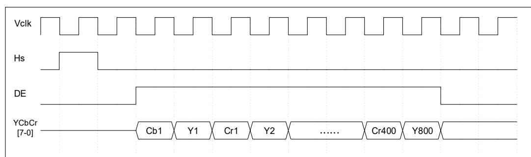
Figure 2-7 8-bit 4:2:2 YCbCr input Video timing
