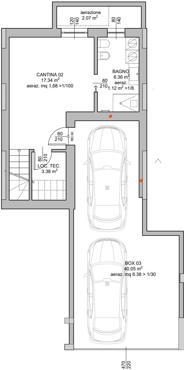
PIANO INTERRATO
