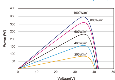
P-V CURVES OF PV MODULE(340W)
