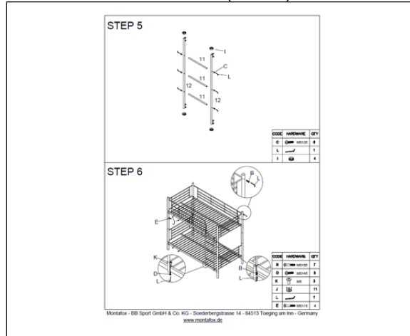
Instruction (view 7)
