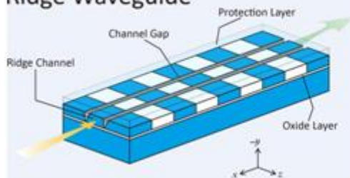
Ridge Waveguide
