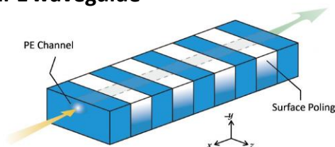
RPE waveguide
