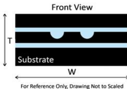
Fig. 2. The geometrical structure and cross-section view of ridge waveguide
