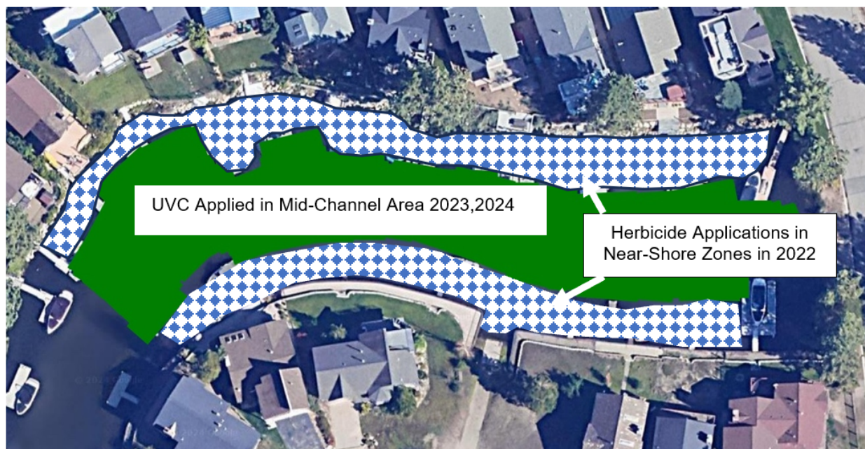
Figure 3-3. Example (aerial view) of CMT Combination site: UVC was used in mid-channel area (Years 2 and 3); Endothall or Triclopyr was applied to the near-shore zone area in 2022.
