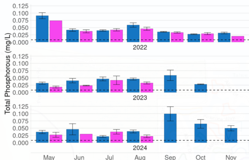
Figure 5-19. TP in UVC Only sites 22 and 24 in CMT Years 1, 2, 3.
