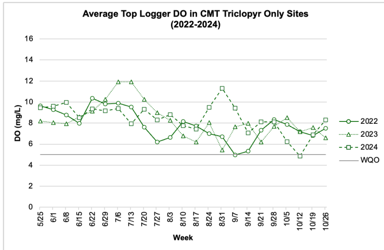
Figure 5-10. DO during the CMT in Triclopyr Only sites: Left = near surface; Right= near bottom. Horizontal black line shows 5 mg/L level.
