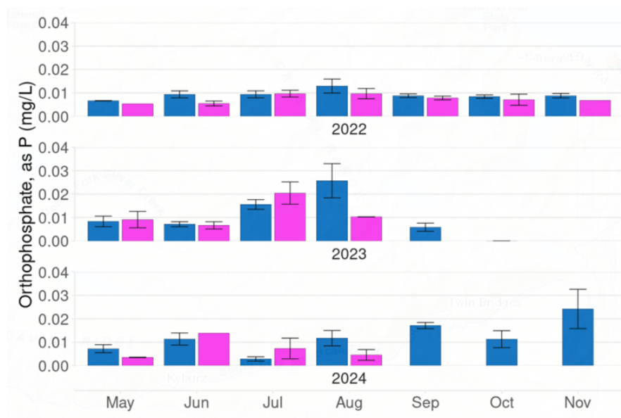
Figure 5-17. OP in UVC Only sites 22 and 24 CMT Years 1,2,3.
