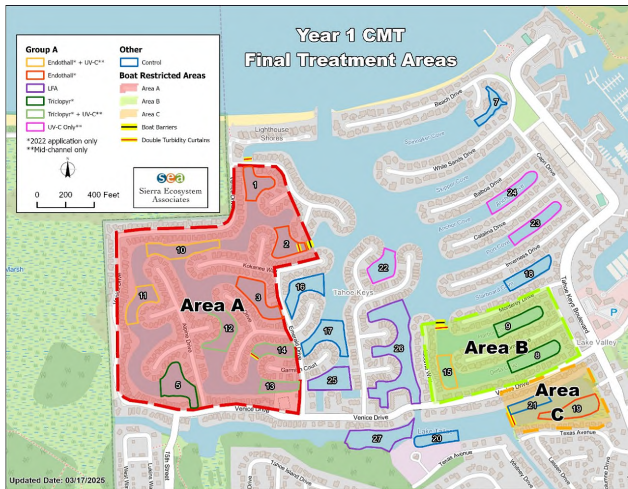
Figure 3-4. Boating restricted areas (A, B, C) during deployment of turbidity curtains. Note: At Sites 1, 3, 13, and 14, culvert plugs were installed to prevent water movement in or out of the Sites into untreated areas or toward Lake Tahoe.
