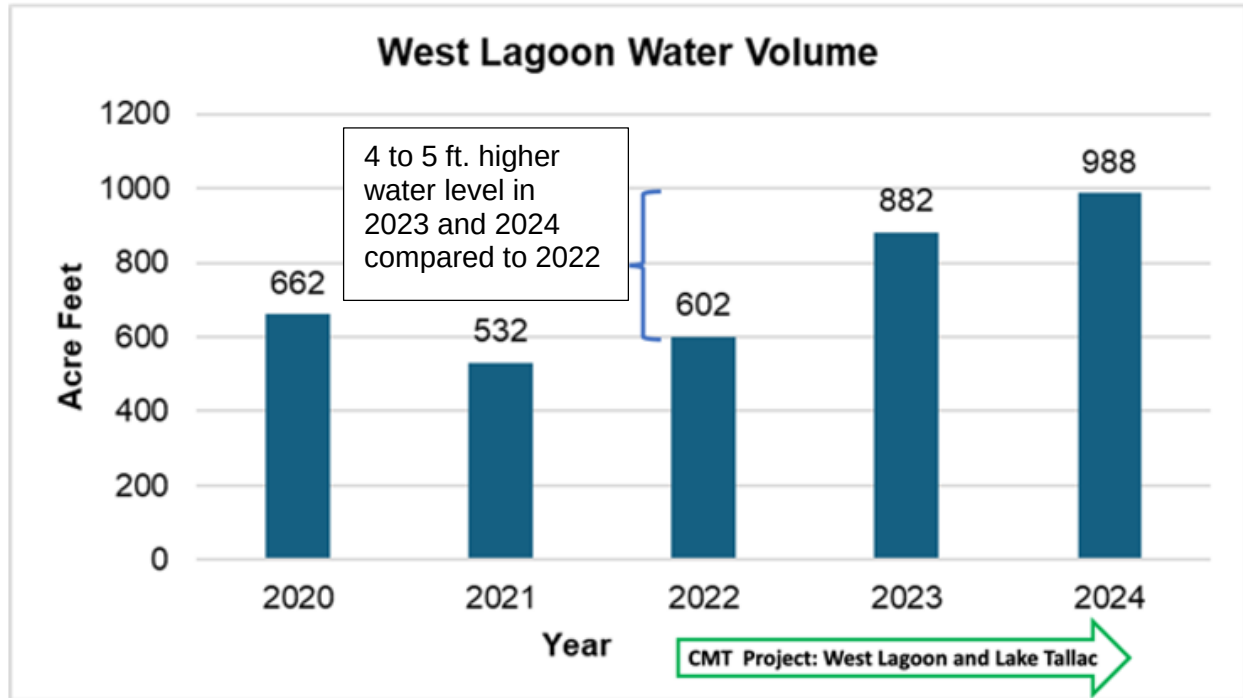
Figure 11-1. Water levels and water volume in the Tahoe Keys West Lagoon.
