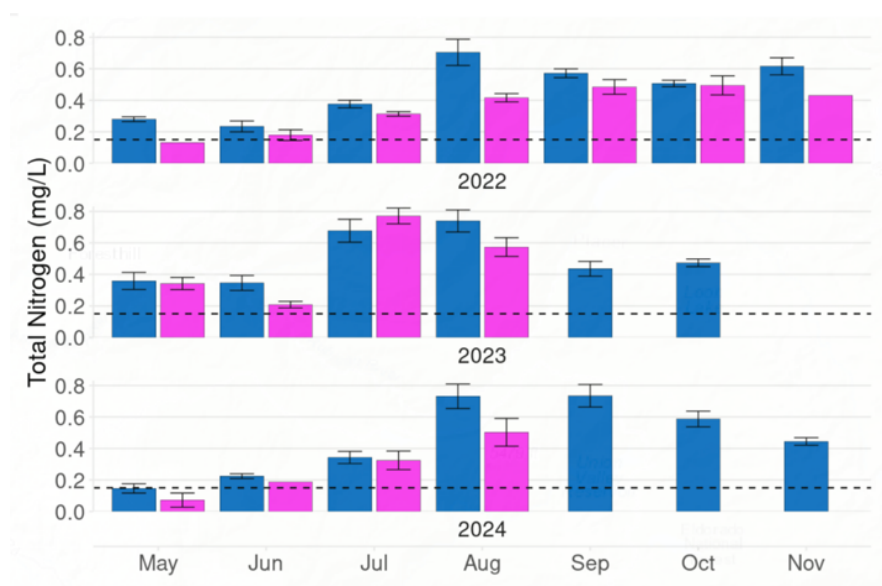
Figure 5-18. TN in UVC Only sites 22 and 24 CMT Years 1,2,3.
