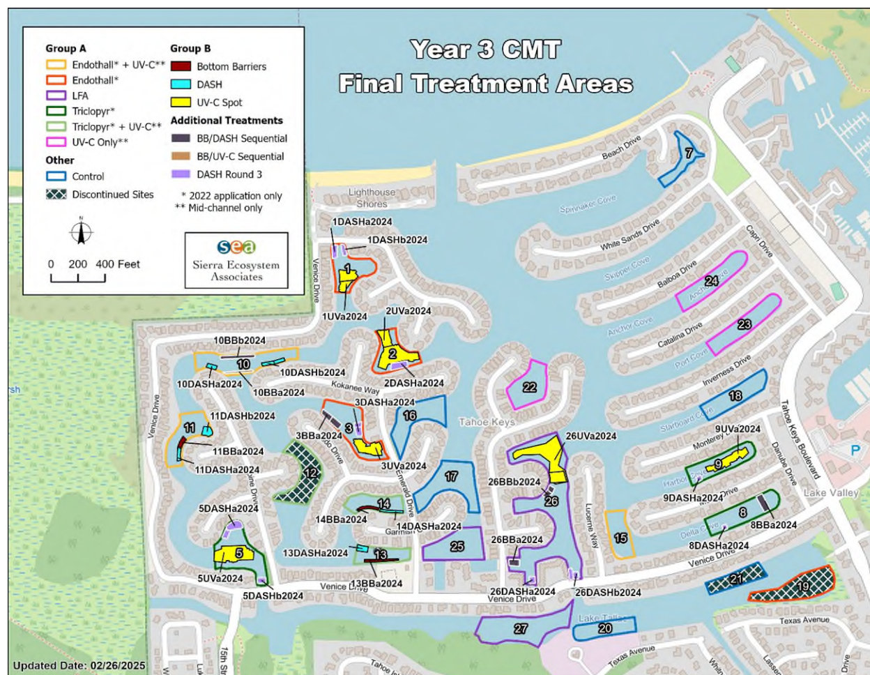
Figure 3-8. CMT Group B areas in Year 3 (2024). Note the map also shows Year 1 (2022) Herbicide applications sites and UVC Only sites
