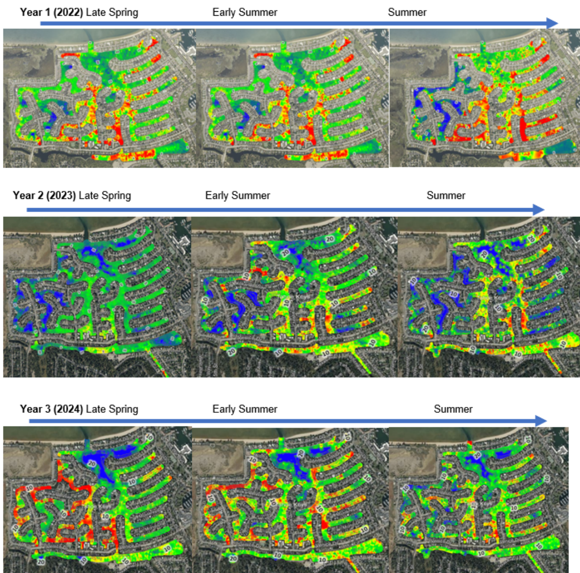
Figure 6-8. Heat maps showing abundance (Biovolume) of AIP in Years 1, 2 and 3: Late Spring, Early Summer, and Summer.
