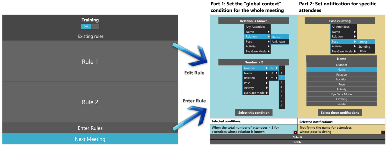
Figure 1: Interface for rule-based programming. Users can create different meeting contexts (Part 1). For each context, a set of notification rules can be defined (Part 2). For example, there may be different notification rules based on meeting size (context).
