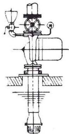
立式給水用 Vertical Mounting
