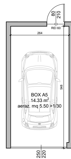
PIANO INTERRATO
