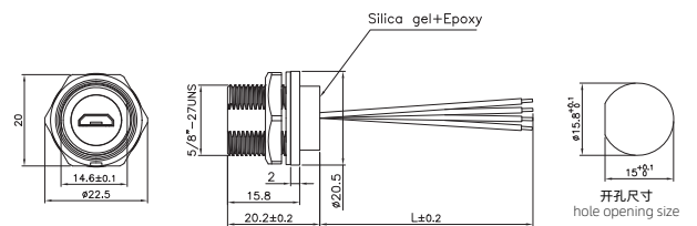
MICRO USB母带电子线板后插座(螺纹) MICRO USB Female Back Mount Receptacle with wire(Threaded)
