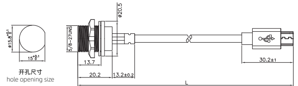
MICRO USB母/公带线板后插座(螺纹) MICRO USB Male to Female Back mount Receptacle Overmolded Cable(Threaded)
