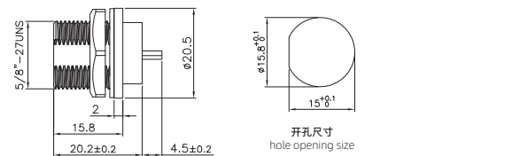
MICRO USB母/母板后插座(螺纹) MICRO USB Female to Female Back Mount Receptacle(Threaded)
