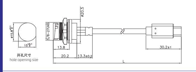
TYPE C母/公带线板后插座(卡扣) TYPE C Male to Female Back mount Receptacle Overmolded Cable(Bayonet)
