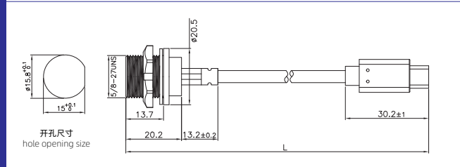
TYPE C母/公带线板后插座(螺纹) TYPE C Male to Female Back mount Receptacle Overmolded Cable(Threaded)
