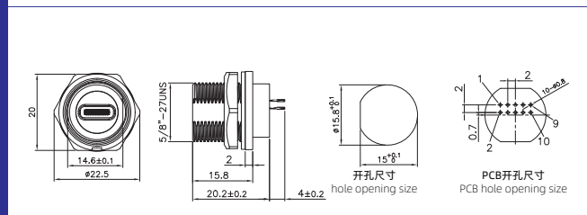
TYPE C母PCB板后插座(螺纹) TYPE C Female Back Mount PCB Receptacle(Threaded)
