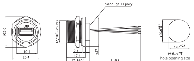
USB 3.0母带电子线板后插座(螺纹) USB 3.0 Female Back Mount Receptacle with wire(Threaded)
