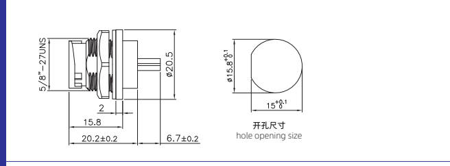
TYPE C母/母板后插座(卡扣) TYPE C Female to Female Back Mount Receptacle(Bayonet)
