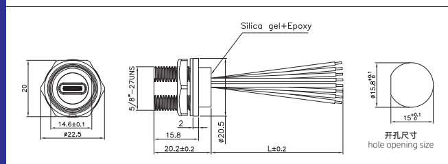
TYPE C母带电子线板后插座(螺纹) TYPE C Female Back Mount Receptacle with wire(Threaded)
