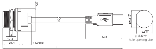
USB 3.0母/公带线板后插座(螺纹) USB 3.0 Female Receptacle to Male Overmolded with Cable (Threaded)
