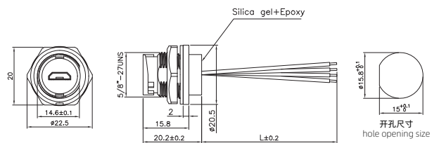
MICRO USB母带电子线板后插座(卡扣) MICRO USB Female Back Mount Receptacle with wire(Bayonet)
