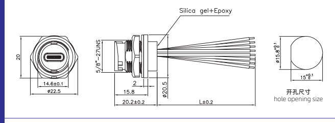
TYPE C母带电子线板后插座(卡扣) TYPE C Female Back Mount Receptacle with wire(Bayonet)
