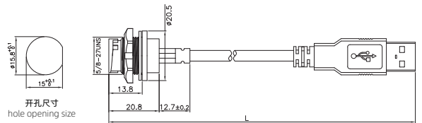
MICRO USB母/USB2.0公带线板后插座(卡扣) MICRO USB Female Back mount Receptacle to USB 2.0 Male Overmolded Cable(Bayonet)
