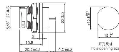
MICRO USB母/母板后插座(卡扣) MICRO USB Female to Female Back Mount Receptacle(Bayonet)
