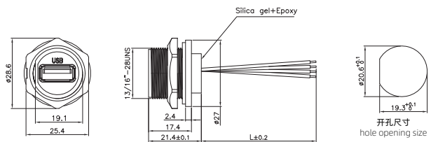
USB 2.0母带电子线板后插座(螺纹) USB 2.0 Female Back Mount Receptacle with wire(Threaded)
