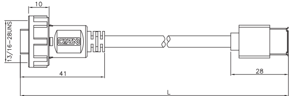
USB 2.0公/母成型直式插头(螺纹) USB 2.0 Female to Male Overmolded with Cable(Threaded)
