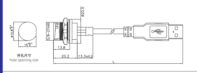
TYPE C母/USB3.0公带线板后插座(卡扣) TYPE C Female Back mount Receptacle to USB 3.0 Male Overmolded Cable(Bayonet)
