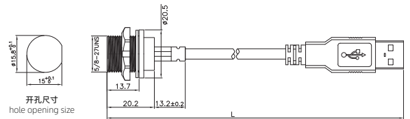
MICRO USB母/USB2.0公带线板后插座(螺纹) MICRO USB Female Back mount Receptacle to USB 2.0 Male Overmolded Cable(Threaded)
