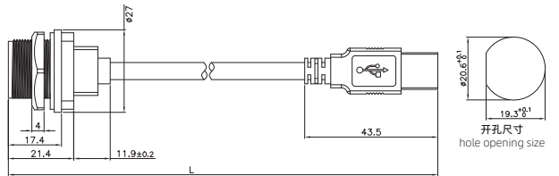
USB 2.0母/公带线板后插座(螺纹) USB 2.0 Female Receptacle to Male Overmolded with Cable (Threaded)
