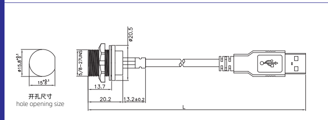
TYPE C母/USB3.0公带线板后插座(螺纹) TYPE C Female Back mount Receptacle to USB 3.0 Male Overmolded Cable(Threaded)
