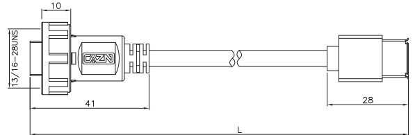
USB 3.0公/母成型直式插头(螺纹) USB 3.0 Female to Male Overmolded with Cable(Threaded)
