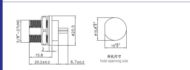
TYPE C母/母板后插座(螺纹) TYPE C Female to Female Back Mount Receptacle(Threaded)
