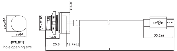
MICRO USB母/公带线板后插座(卡扣) MICRO USB Male to Female Back mount Receptacle Overmolded Cable(Bayonet)
