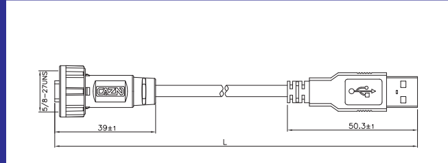
TYPE C公/USB3.0公成型直式插头(螺纹) TYPE C Male to USB 3.0 Male Overmolded Cable(Threaded)
