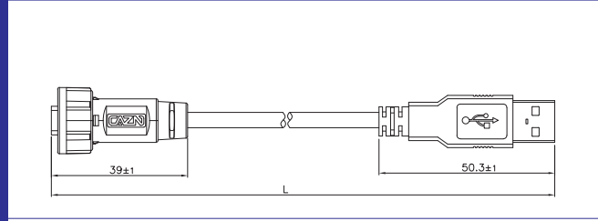
TYPE C公/USB3.0公成型直式插头(卡扣) TYPE C Male to USB 3.0 Male Overmolded Cable(Bayonet)
