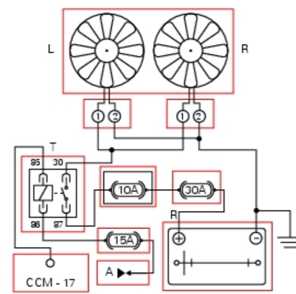
Spal Fan Wiring Diagram Single - Complete Wiring Schemas
