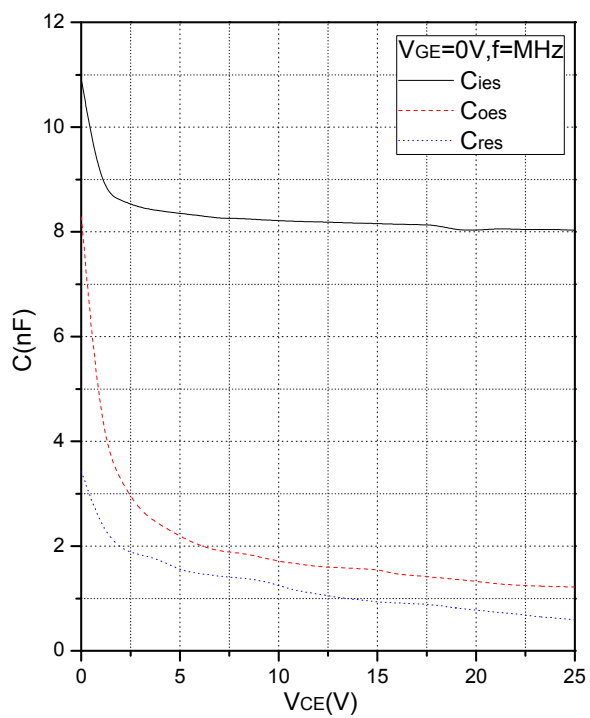
Fig.15 Capacitance Characteristics
