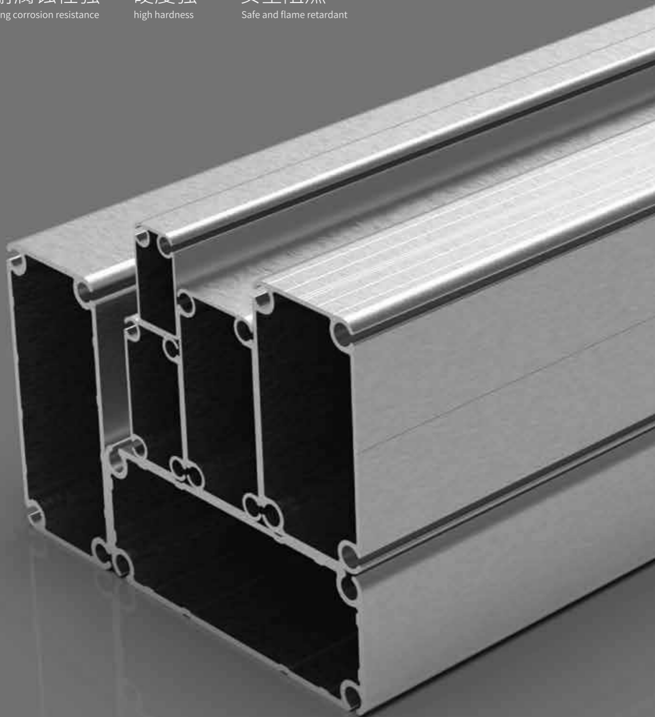
12M Tent: 121x68mm (适用于跨度为12M的篷房) (Suitable for tents with a span of 12M)
