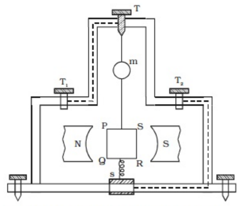
Fig 3.26 Moving coil galvanometer
